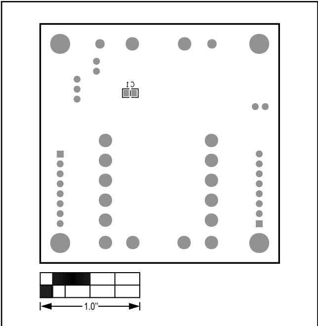
MAX14851 EV Kit—PCB Silkscreen Bottom Side
