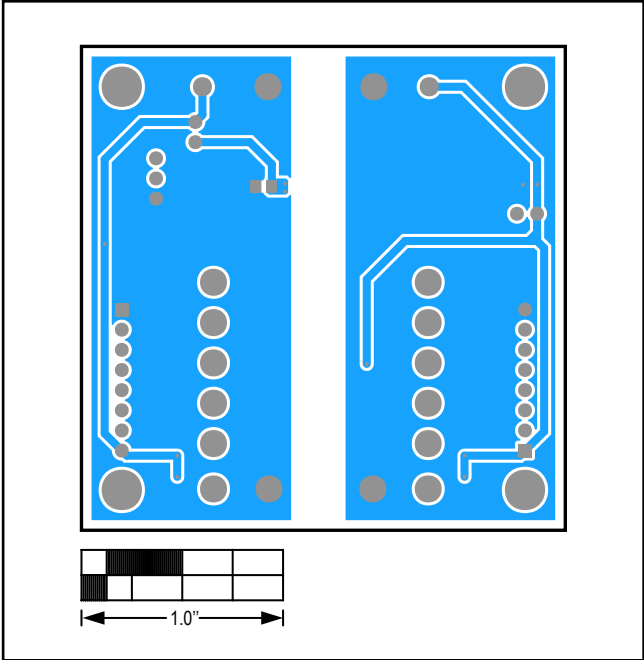
MAX14851 EV Kit—PCB Layout Bottom Side
