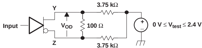
Figure 12. Driver VDO Test Circuit
