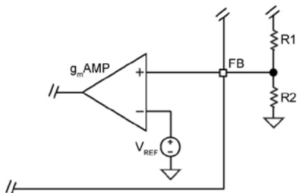
Figure 9. Voltage-Divider Configuration
