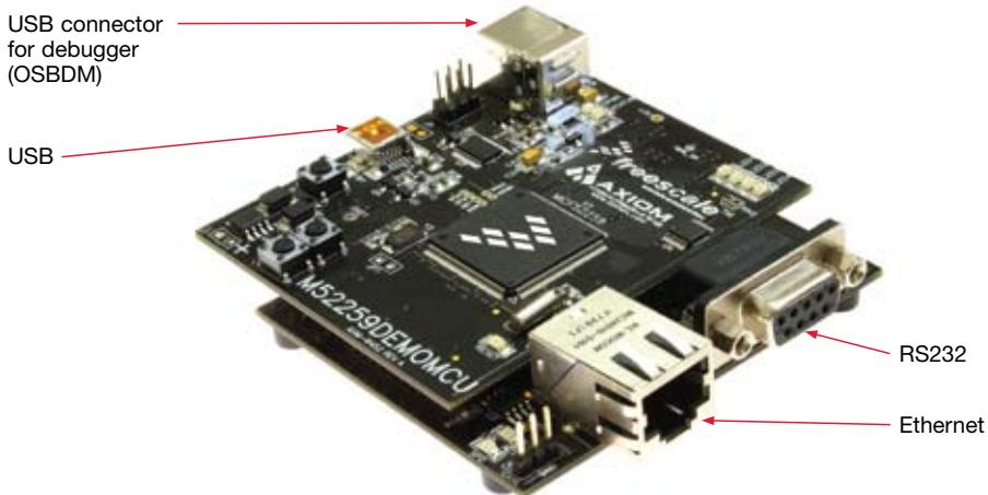
Figure 1. M52259DEMOKIT
