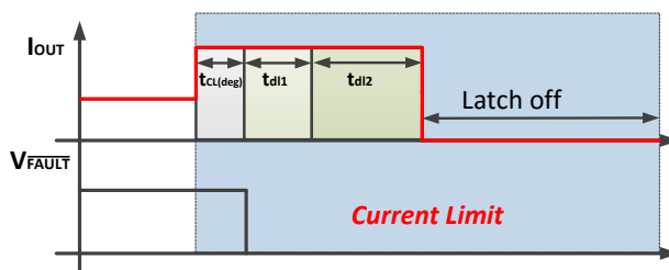
Figure 16. Latch-Off-Mode Example
