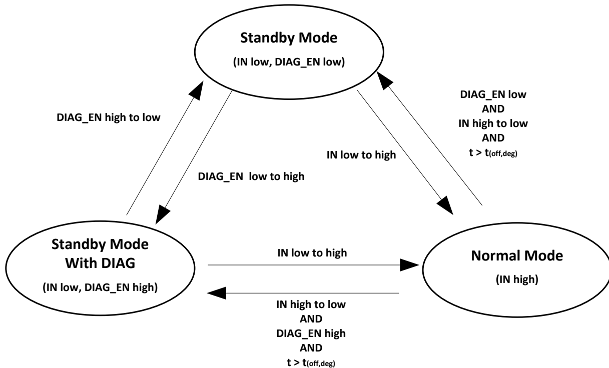
Figure 31. Working Modes
