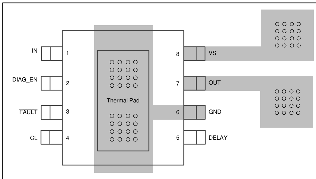
Figure 35. Layout Example
