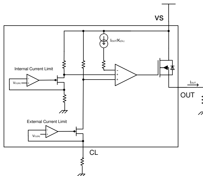
Figure 12. Current Limit
