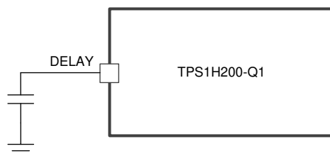
Figure 15. Latch-Off-Mode Connection
