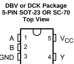
Pin Functions
