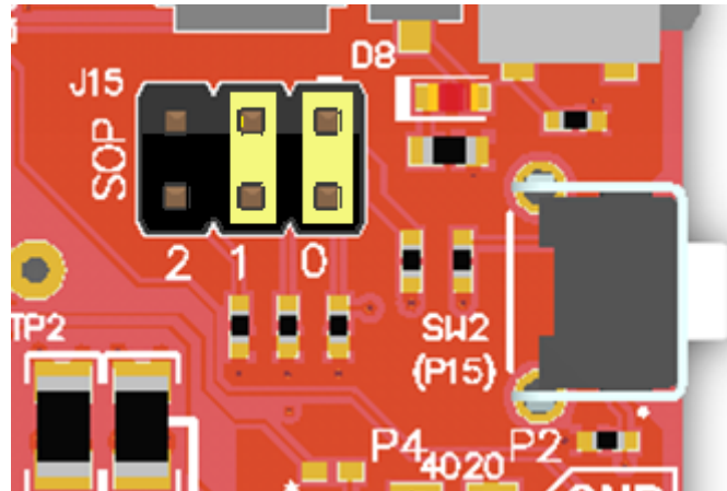
Figure 10. SOP Jumpers Configuration
