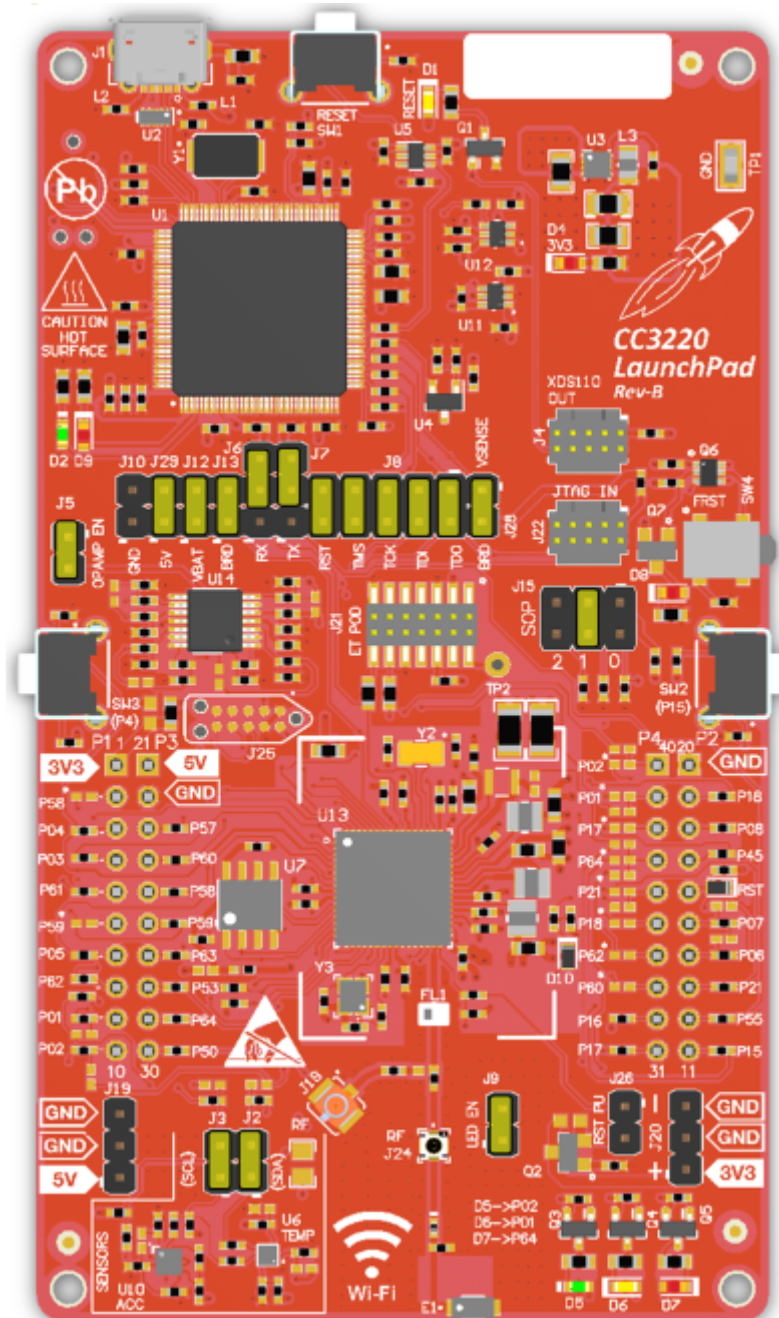
Figure 9. CC3220 Default Jumpers Settings
