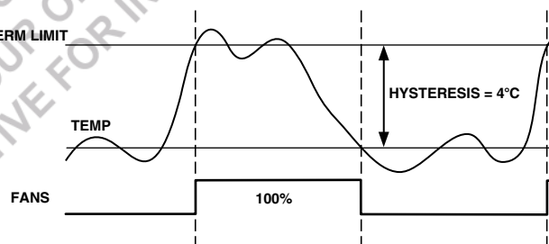
Figure 15. THERM Limit Operation
