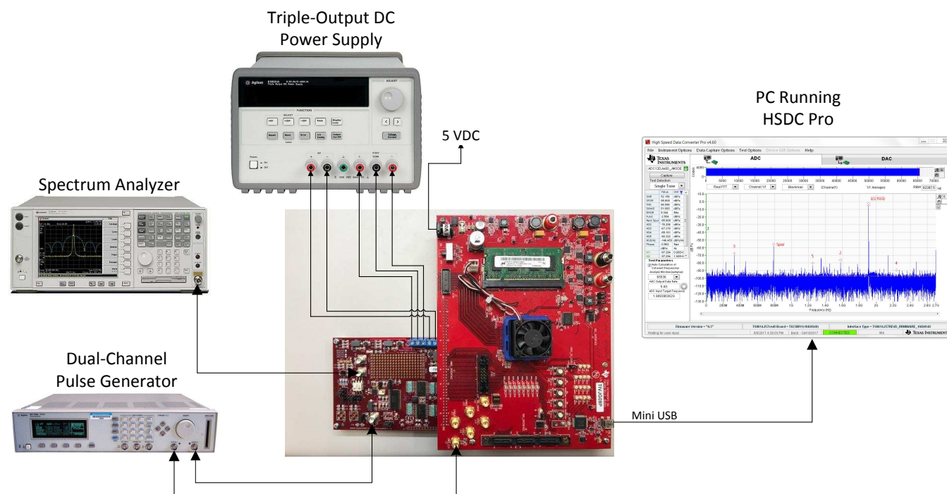
Figure 3. Quick-Start Test Setup
