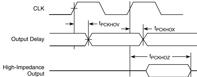
Figure 32. PCI Output AC Timing Diagram
