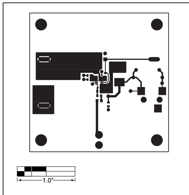
Figure 3. MAX4336 EV Kit PC Board Layout—Component Side
