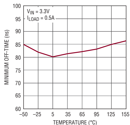
Minimum Off-Time
