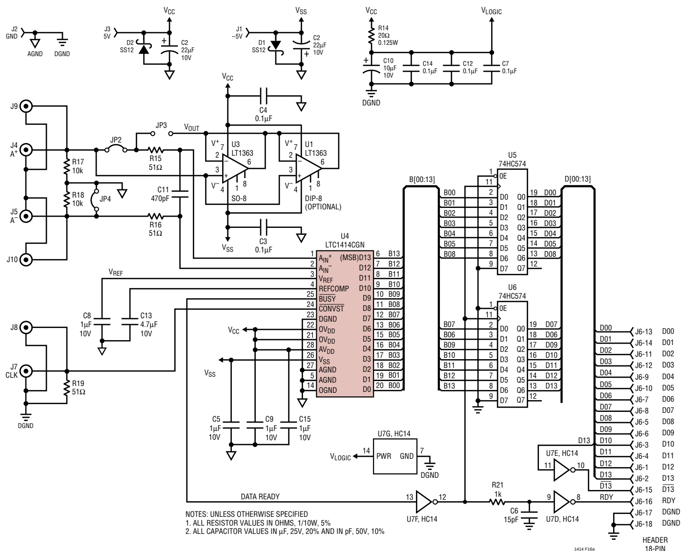
Figure 16a. Evaluation Circuit Schematic
