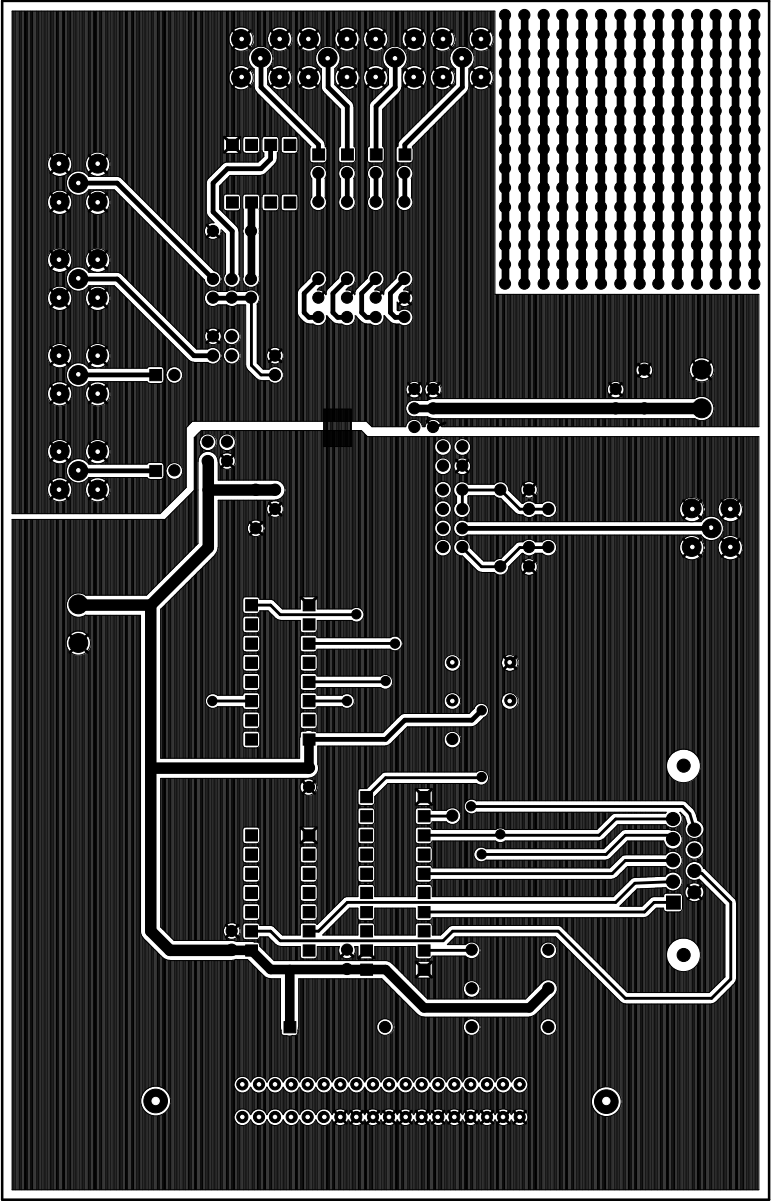
Eval-AD7730LEB (Component Side View) (Solder Side)
