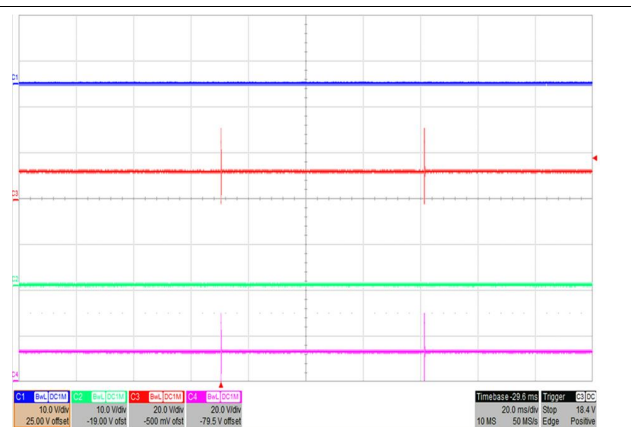
Figure 26. V_{IN} = 390\text{ V} , I_{OUT} = 0\text{ A} , No Gate Drive Under Light Load (VG1, VG2)
