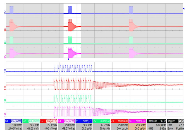
Figure 30. V_{IN} = 410 V, I_{OUT} = 0.3 A, LLC is Operating In Burst Mode
