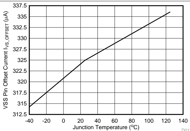
Figure 12. VSS Pin Offset Current vs Temperature
