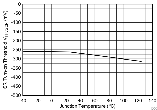
Figure 3. SR Turn-on Threshold Voltage vs Temperature
