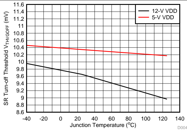
Figure 4. SR Turn-off Threshold Voltages vs Temperature
