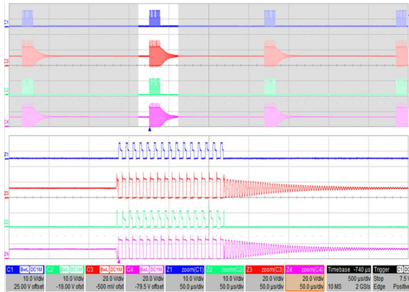
Figure 27. V_{IN} = 390 V, I_{OUT} = 0.3 A, LLC is Operating In Burst Mode
