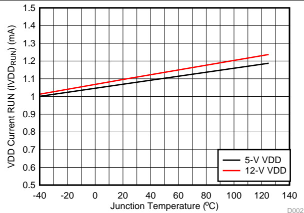
Figure 2. Bias Supply Current vs Temperature (No Switching)
