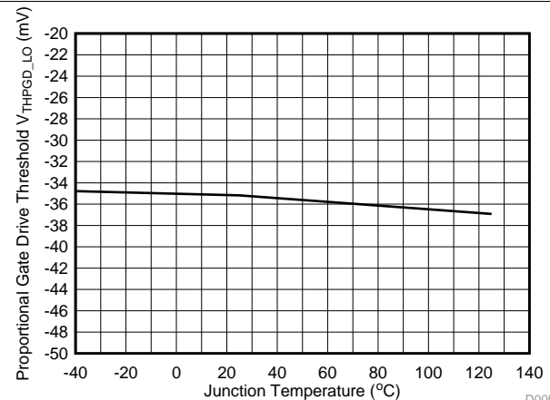
Figure 5. Proportional Gate Drive Threshold vs Temperature
