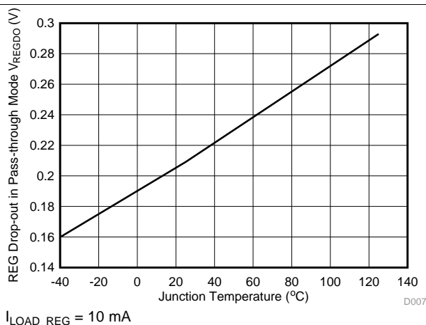
Figure 7. REG Dropout in Pass-through Mode vs Temperature
