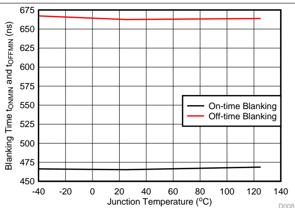
Figure 8. Blanking Time vs Temperature
