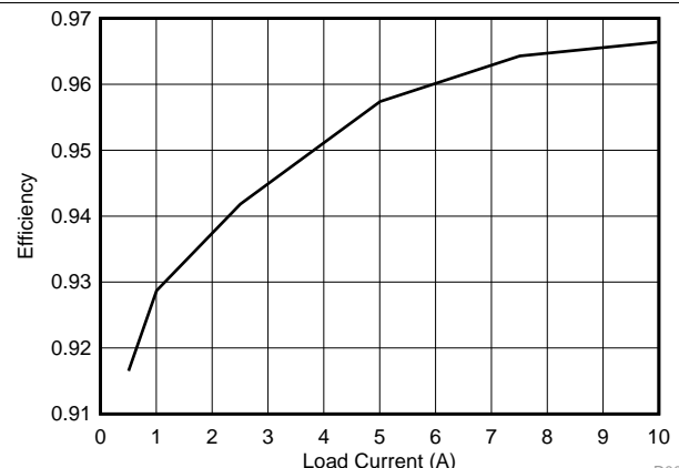
Figure 32. V_{IN} = 390 V, Power Converter System Efficiency Using SR FETs
