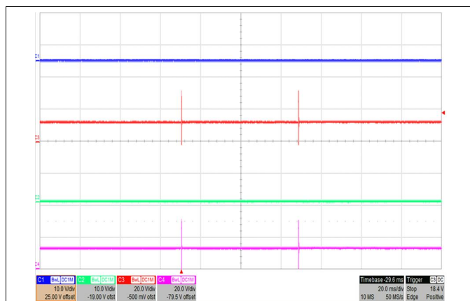
Figure 23. V_{IN} = 340\text{ V} , I_{OUT} = 0\text{ A} , No Gate Drive Under Light Load (VG1, VG2)
