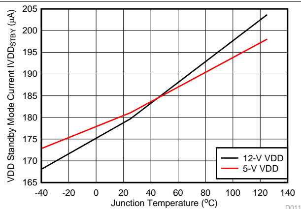
Figure 11. Standby Current vs Temperature
