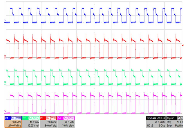
Figure 28. V_{IN} = 390 V, I_{OUT} = 10 A Full Load
