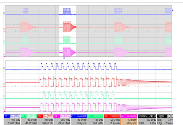
Figure 24. V_{IN} = 340\text{ V} , I_{OUT} = 0.3\text{ A} , LLC is Operating In Burst Mode
