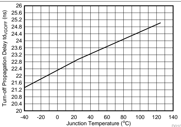
Figure 10. SR Turn-off Propagation Delay vs Temperature
