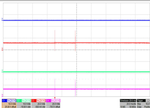
Figure 29. V_{IN} = 410 V, I_{OUT} = 0 A, No Gate Drive Under Light Load (VG1, VG2)
