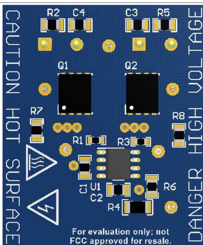
Figure 36. UCC24624EVM-015 (Bottom View)
