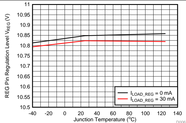
Figure 6. REG Pin Voltage vs Temperature at Different Loading Conditions
