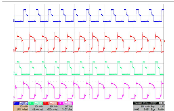
Figure 25. V_{IN} = 340\text{ V} , I_{OUT} = 10\text{ A} Full Load
