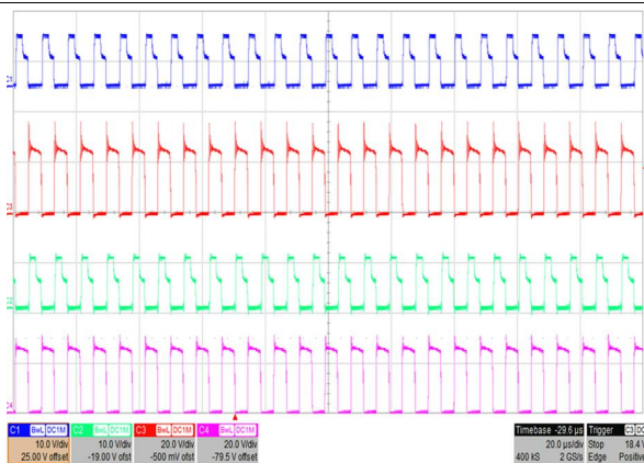
Figure 31. V_{IN} = 410 V, I_{OUT} = 10 A Full Load
