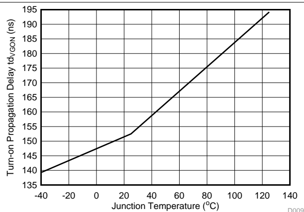
Figure 9. SR Turn-on Delay Time vs Temperature
