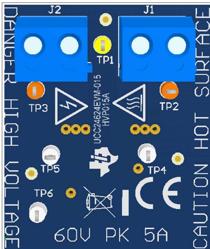
Figure 35. UCC24624EVM-015 (Top View)
