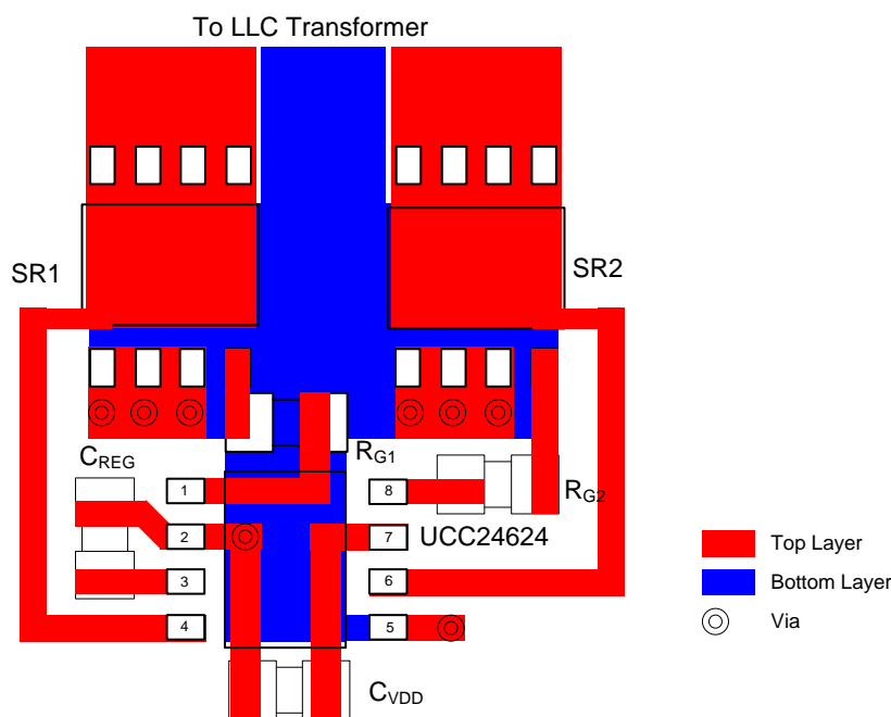
Figure 34. UCC24624 Layout Example
