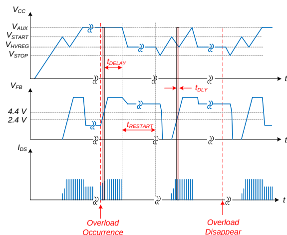
Figure 20. OLP Waveforms
