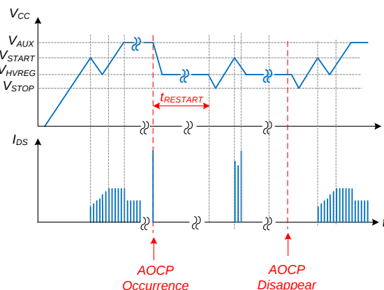
Figure 22. AOCP Waveforms
