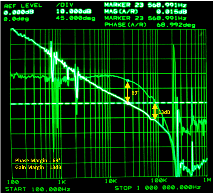
Figure 7. Gain and Phase Margin ( V_{PORT} = 57V , 5V/13A)
