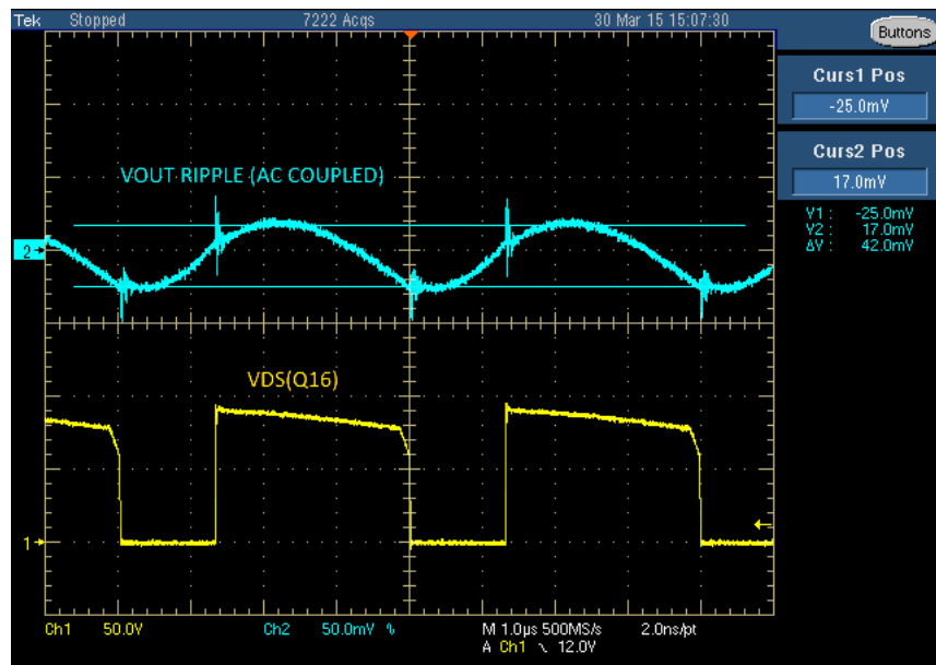
Figure 5. Output Voltage Ripple ( V_{PORT} = 57V , 5V/13A)
