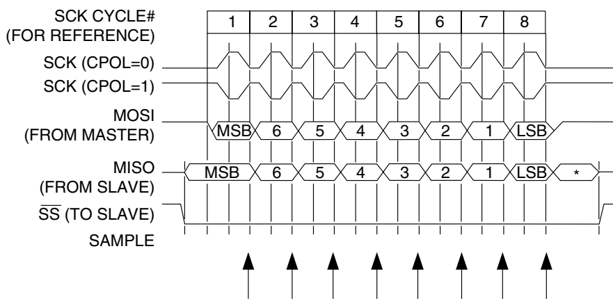
Figure 39. SPI Transfer Format with CPHA = 0 and DORD = 0
