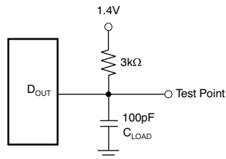
Load Circuit for t_{\text{dDO}} , t_r , and t_f
