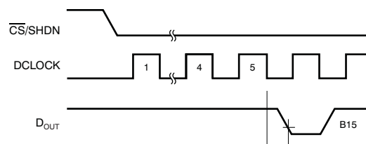
Voltage Waveforms for t_{\text{en}}
