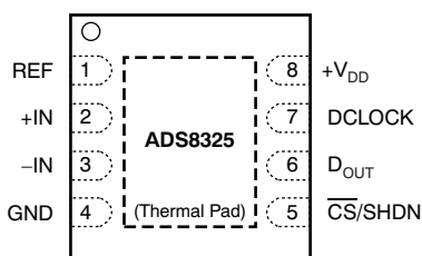
DRB PACKAGE (1) SON (TOP VIEW)
