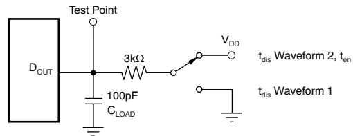
Load Circuit for t_{\text{dis}} and t_{\text{en}}
