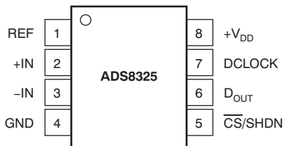
DRB PACKAGE (1) SON (TOP VIEW)
