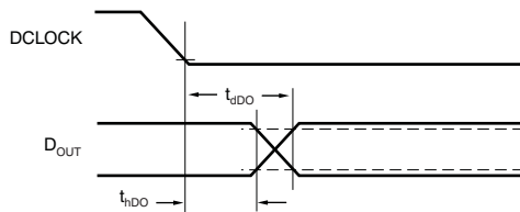
Voltage Waveforms for \text{D}_{\text{OUT}} Delay Times, t_{\text{dDO}}
