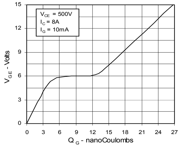
Fig. 8. Gate Charge
