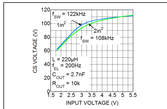
FIGURE 2-6: Peak CS Voltage vs. Input Voltage.
