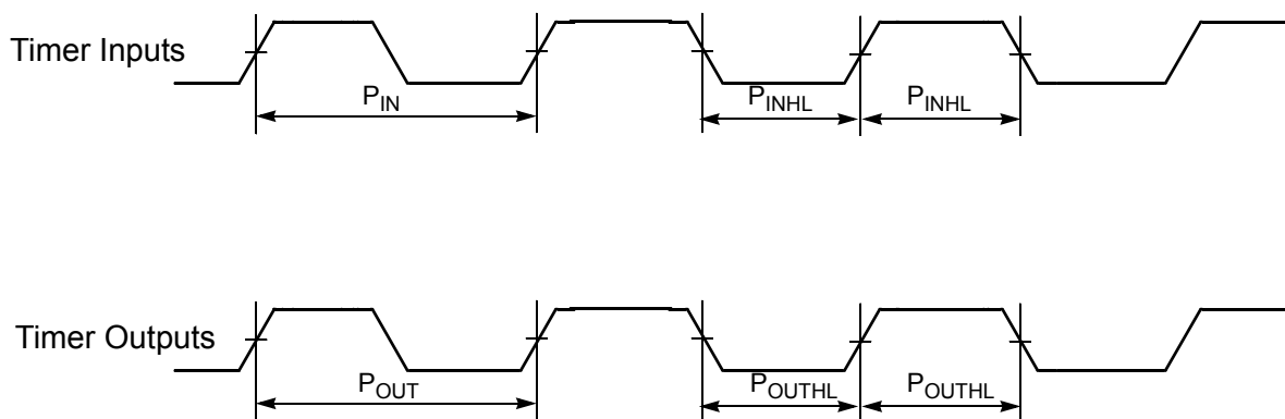
Figure 4-21 Timer Timing
