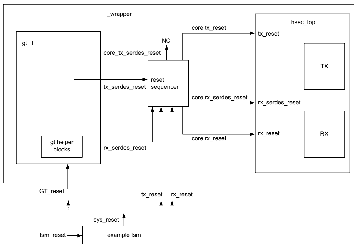
Figure 3-6: Reset Structure
