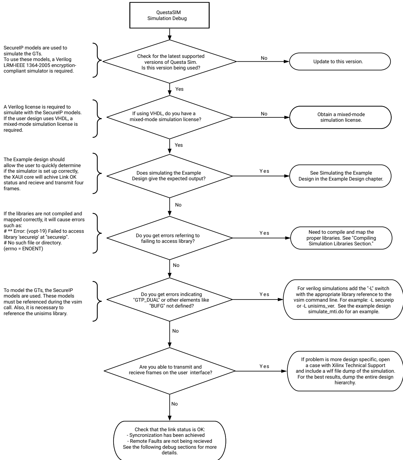
Figure B-1: Mentor Graphics Questasim Advanced Simulator Simulation Debug Flow
