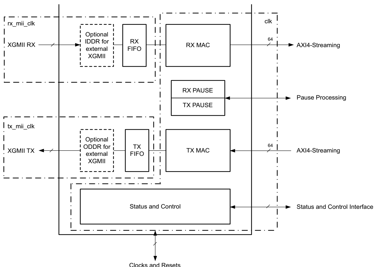
Figure 3-4: Clocking Architecture for the 10G MAC-only Configuration
