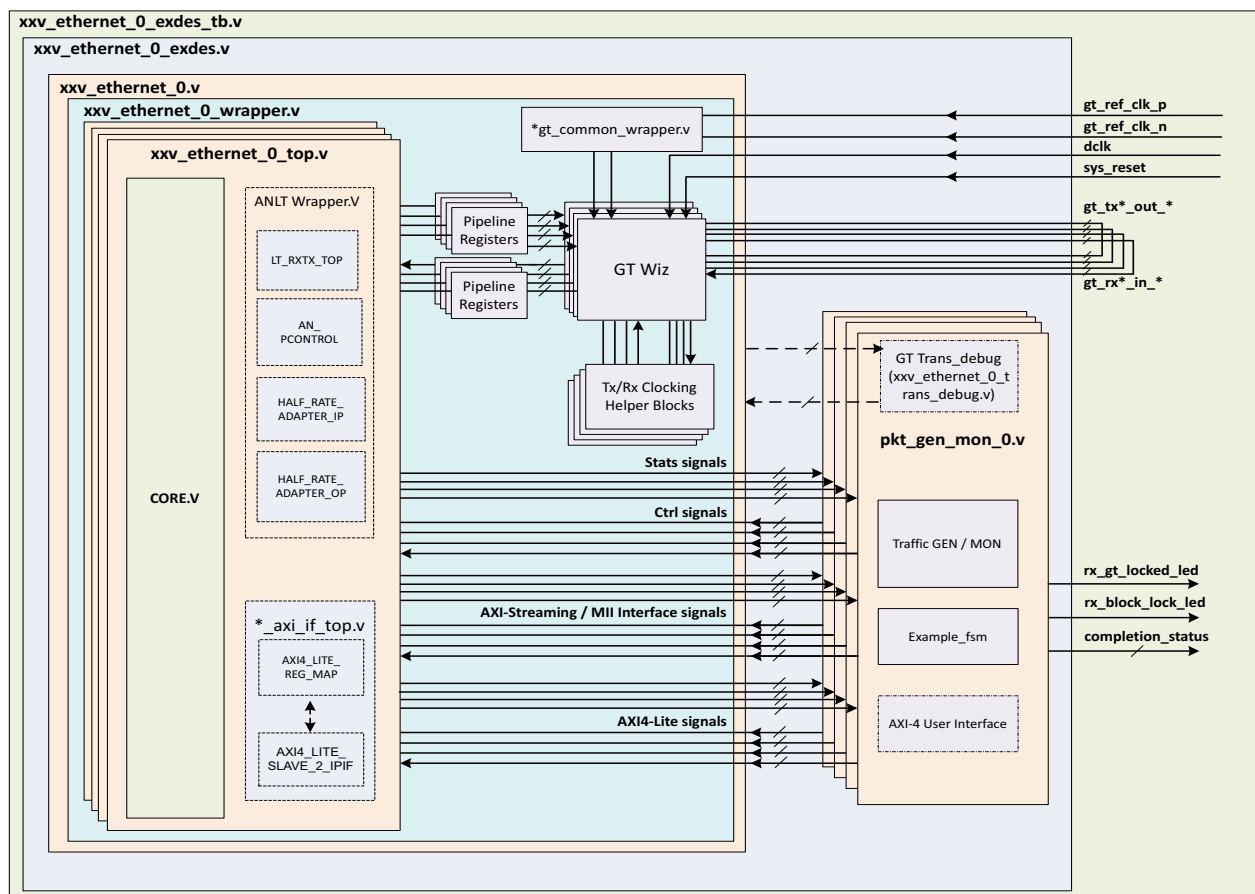
Figure 5-2: Multiple Core Example Design Hierarchy
