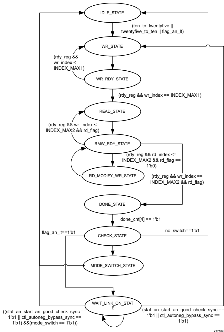
Figure 5-7: State Transition Diagram for Runtime Switchable DRP Operation with AN/LT
