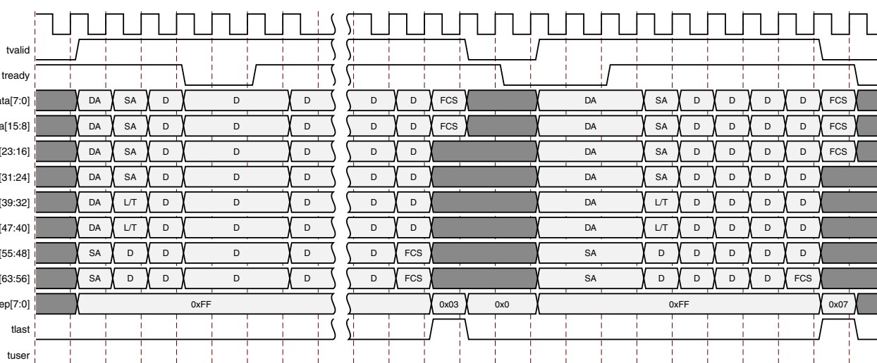
Figure 2-6: Normal Frame Transfer – 64 Bit
