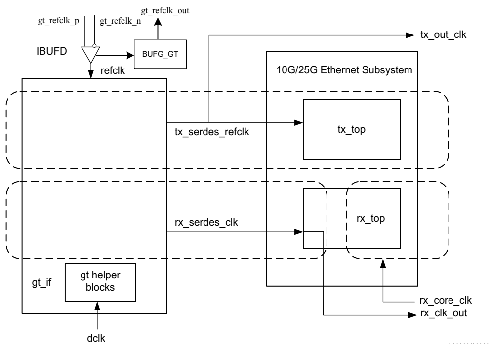
Figure 3-2: 10G/25G MAC with PCS/PMA Clocking
