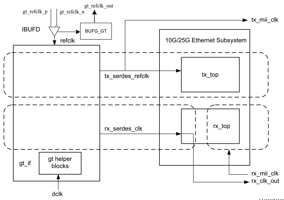
Figure 3-1: PCS/PMA Clocking
