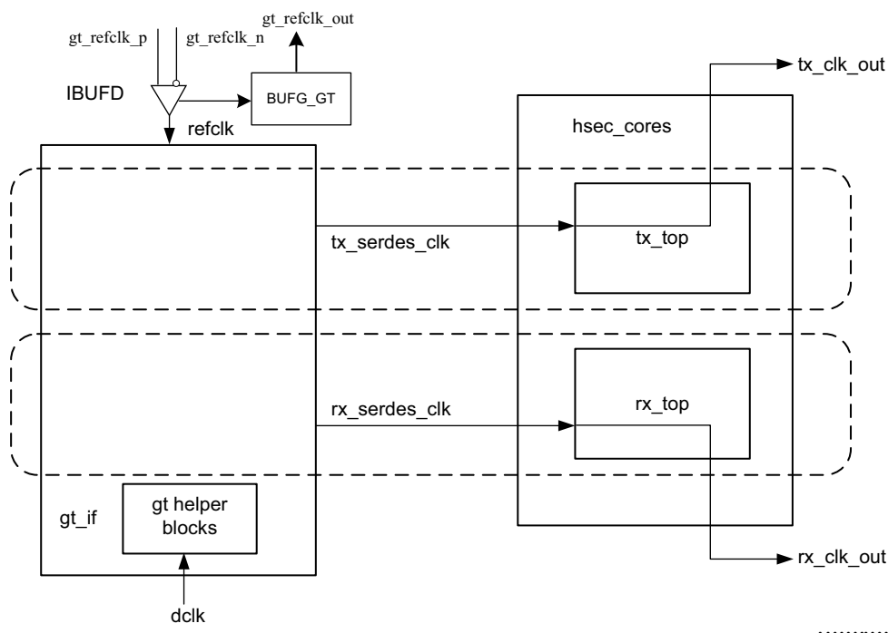
Figure 3-3: Low Latency 10G/25G MAC with PCS/PMA Clocking
