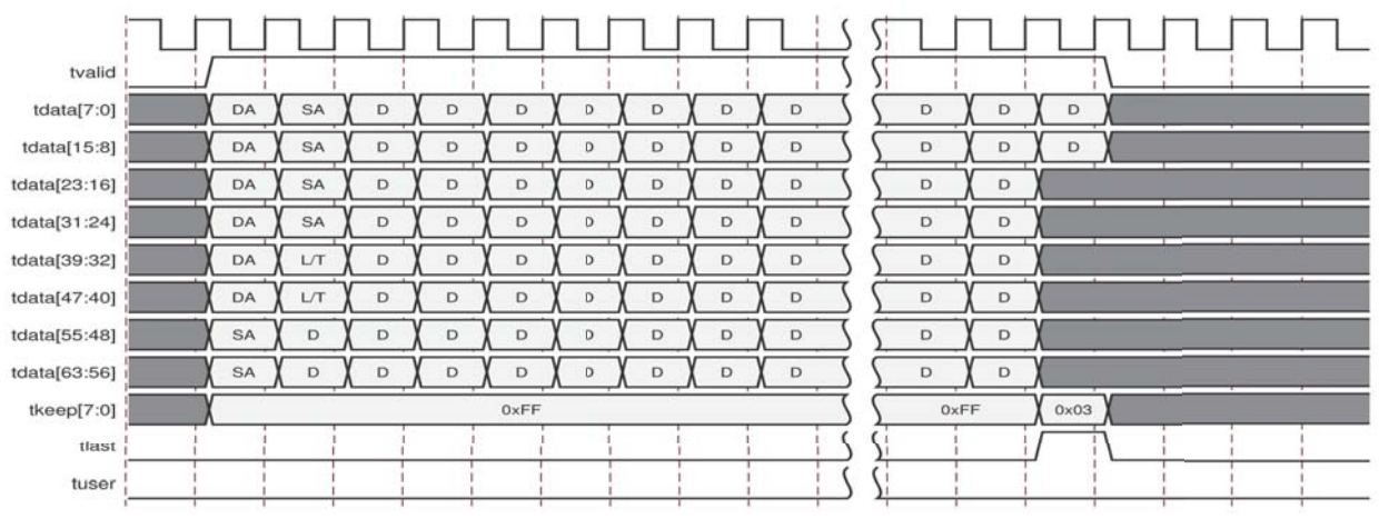
Figure 2-10: Normal Frame Reception – 64 Bits
