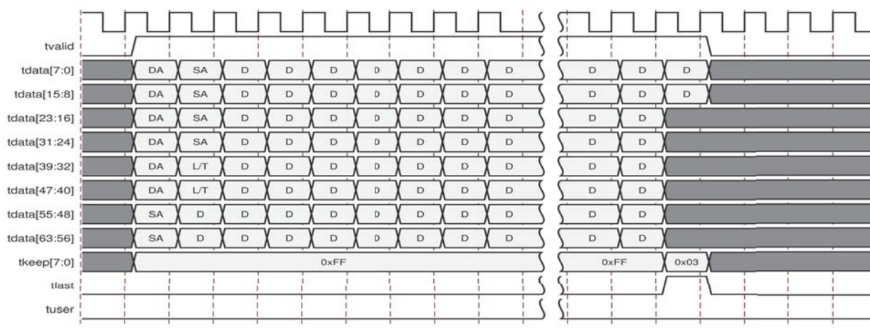
Figure 2-14: Normal Frame Reception – 64 Bits
