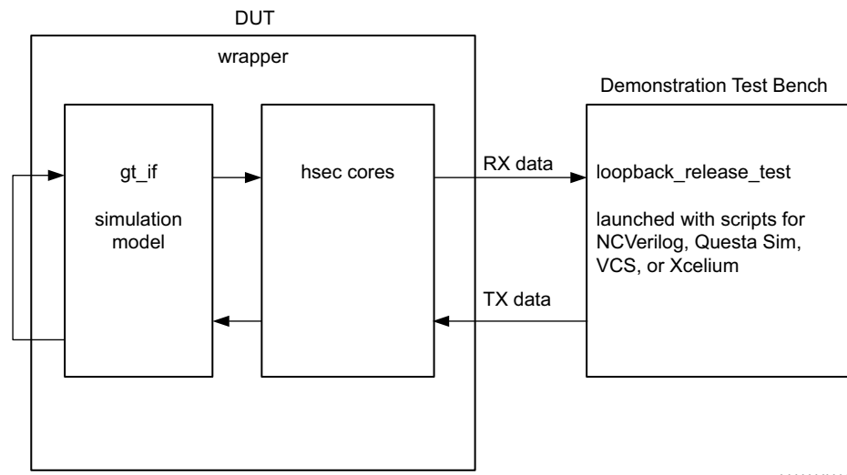
Figure 6-1: Test Bench
