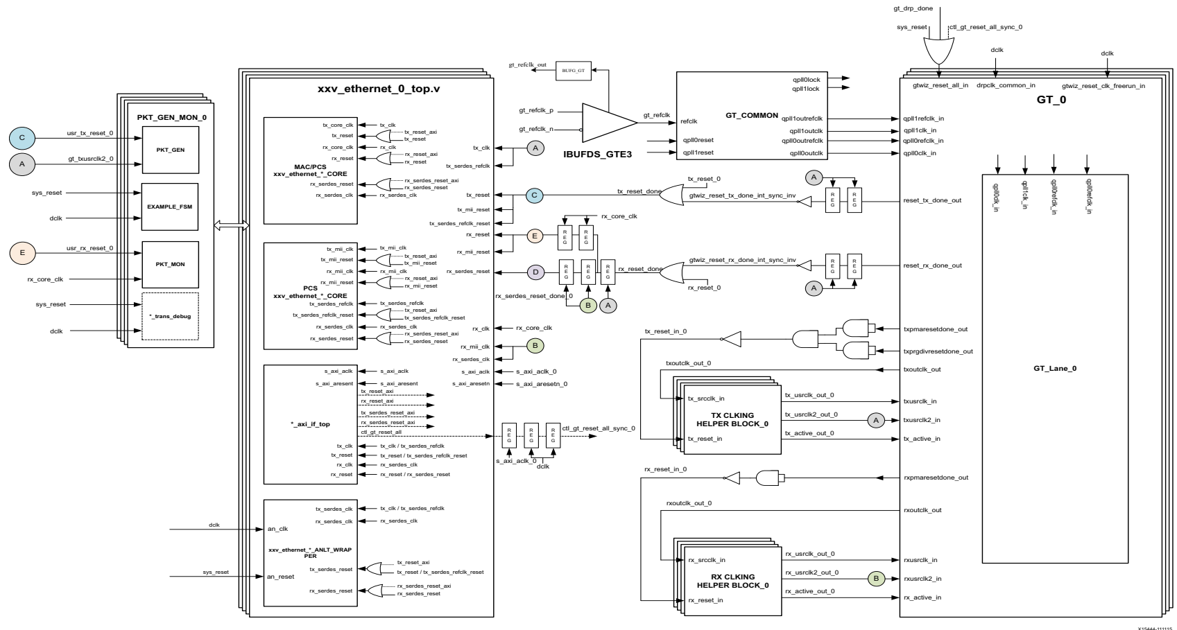
Figure 3-8: Detailed Diagram of Multiple Cores - Asynchronous Clock Mode
