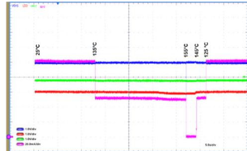
Figure 4: Thermal management
