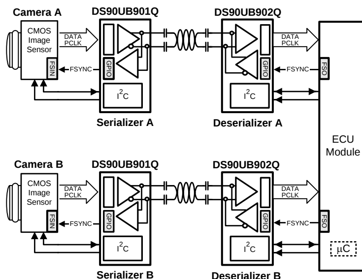
Figure 32. Synchronizing Multiple Cameras
