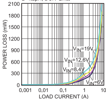
Power Loss
