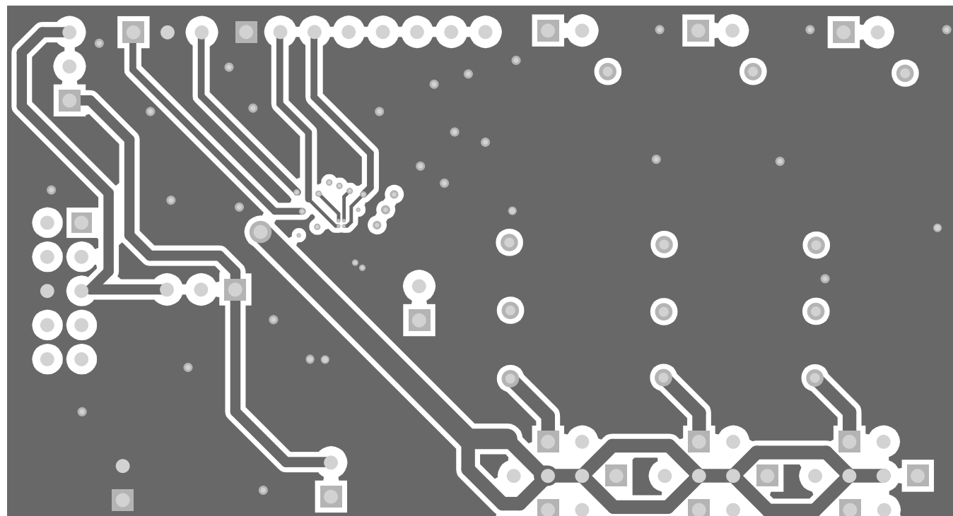
Figure 3. Mid Layer 1
