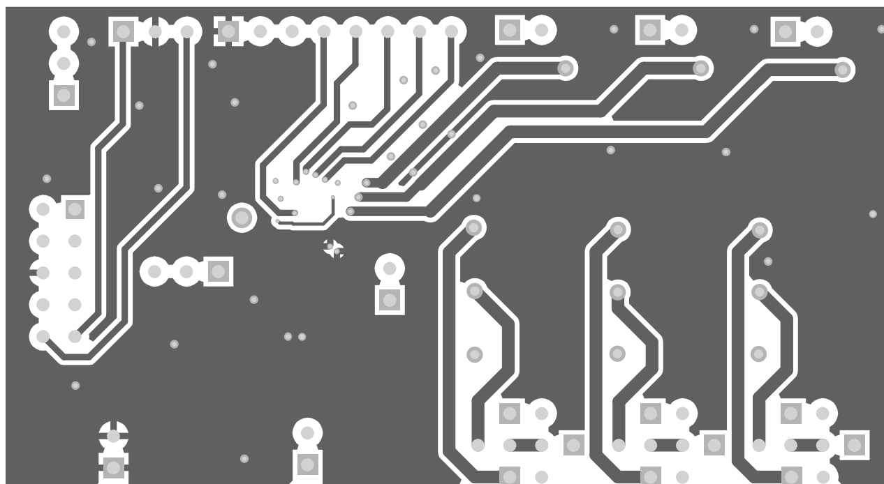
Figure 4. Mid Layer 2
