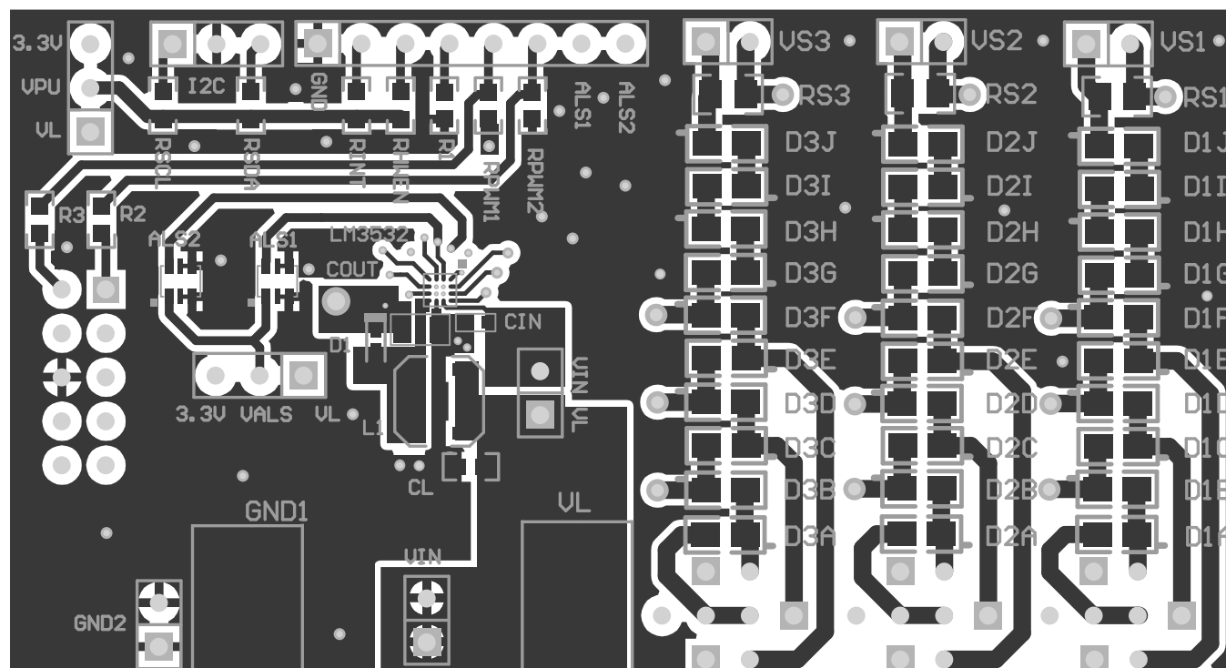
Figure 2. Top Layer
