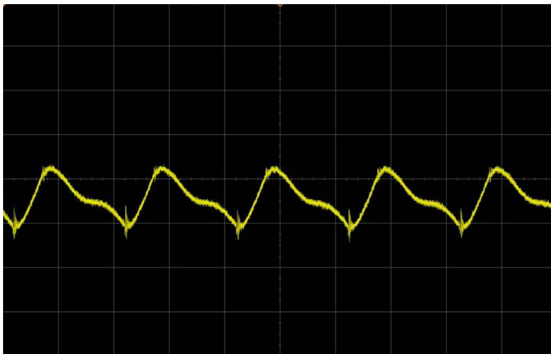
Figure 3. Output Ripple at 48V IN and 11A OUT (50mV, 2μs/DIV, 20MHz)
