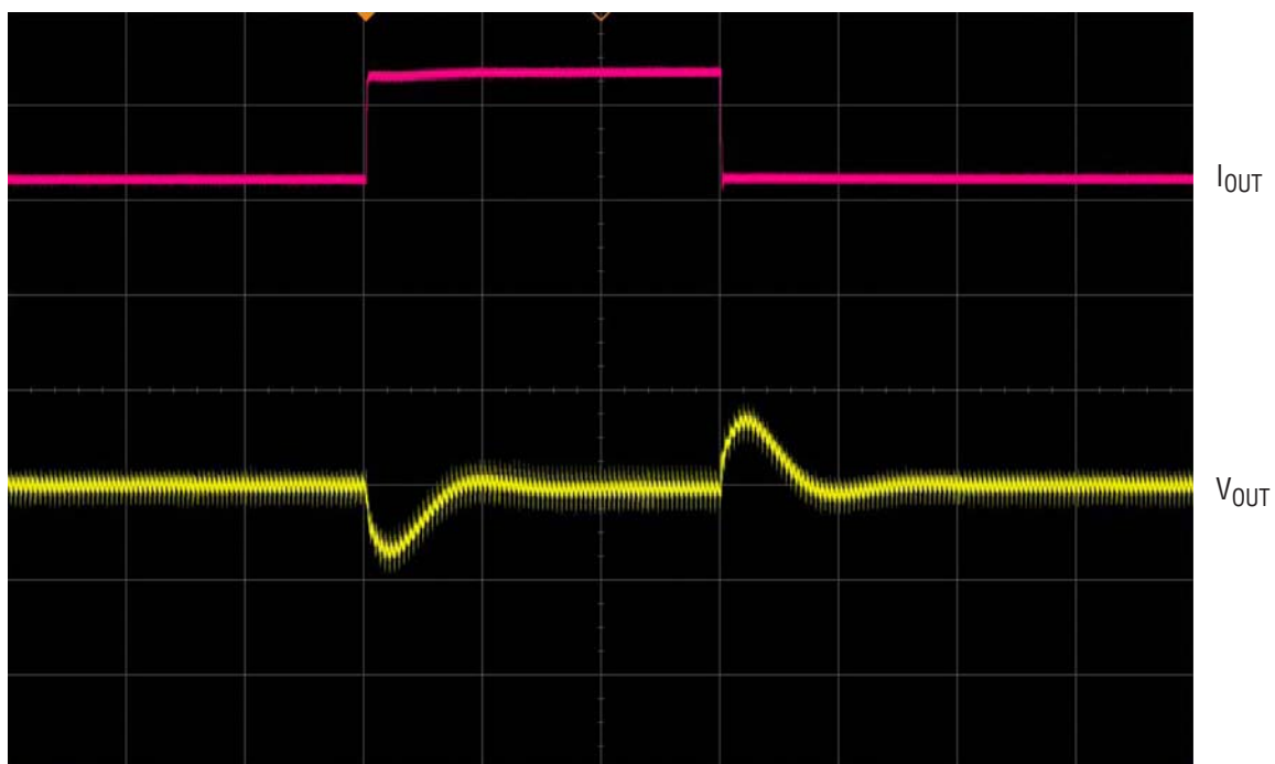
Figure 4. Transient Response Waveform at 48V IN and 6 – 12A OUT (5A, 500mV, 100μs/DIV)
