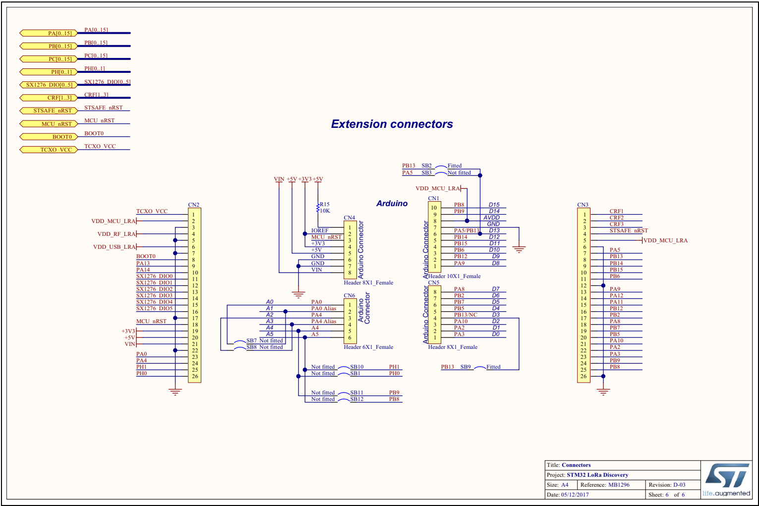
Figure 15. Connectors
