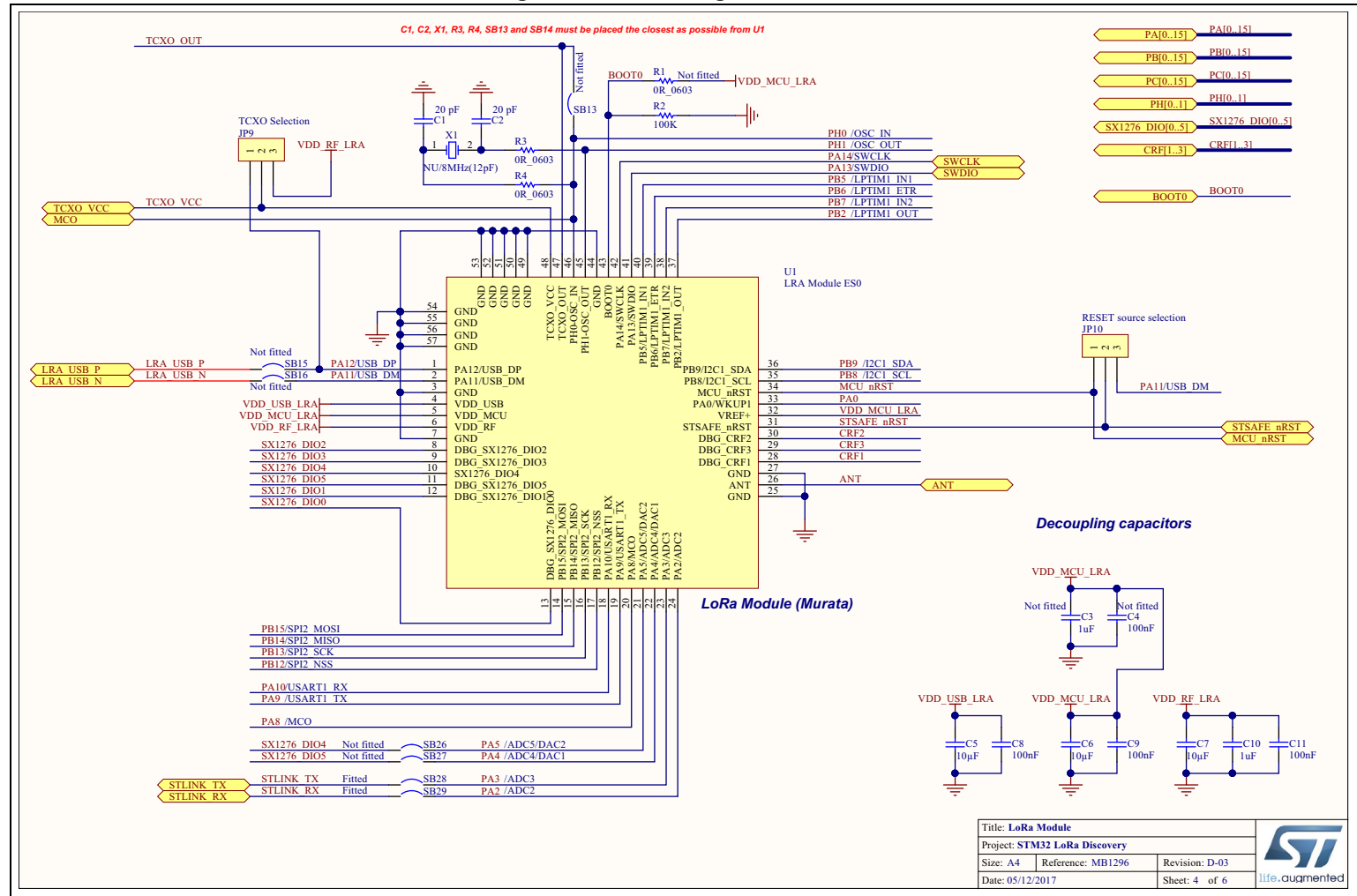
Figure 13. LoRa®/Sigfox™ module
