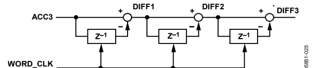
Figure 27. Differentiator
