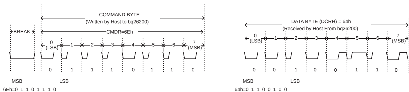
Figure 4. Communication Sequence
