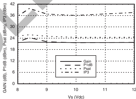
Gain, Power & OIP3 vs. Supply Voltage for Constant I_{CC}=110\text{ mA} @ 850 MHz
