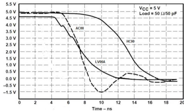
Figure 5. Typical Application Curve
