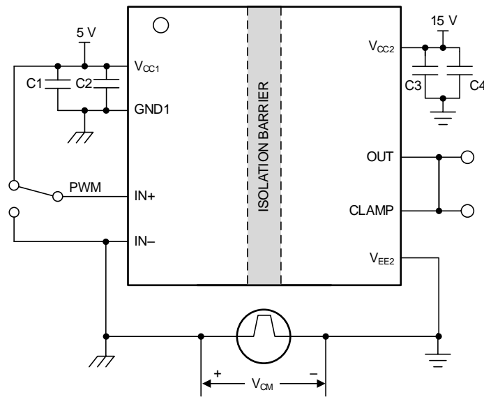
Figure 45. CMTI Test Circuit for Miller Clamp (UCC53x0M)
