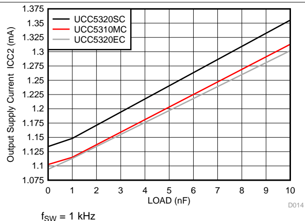
Figure 22. I_{CC2} Supply Current vs Load Capacitance
