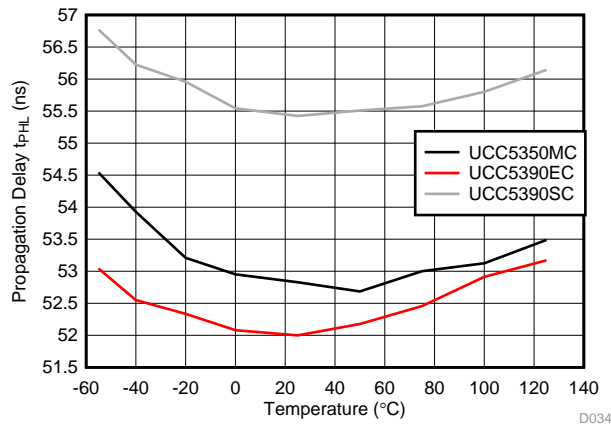
Figure 35. Propagation Delay t_{\text{PHL}} vs Temperature
