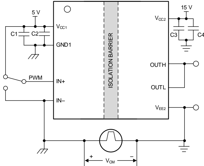
Figure 44. CMTI Test Circuit for Split Output (UCC53x0S)
