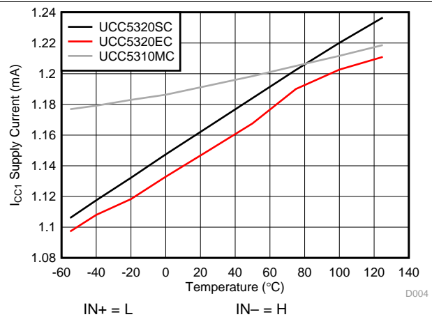
Figure 10. I_{CC1} Supply Current vs Temperature
