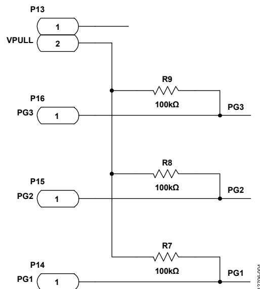
Figure 4. Power-Good Pin Circuit
