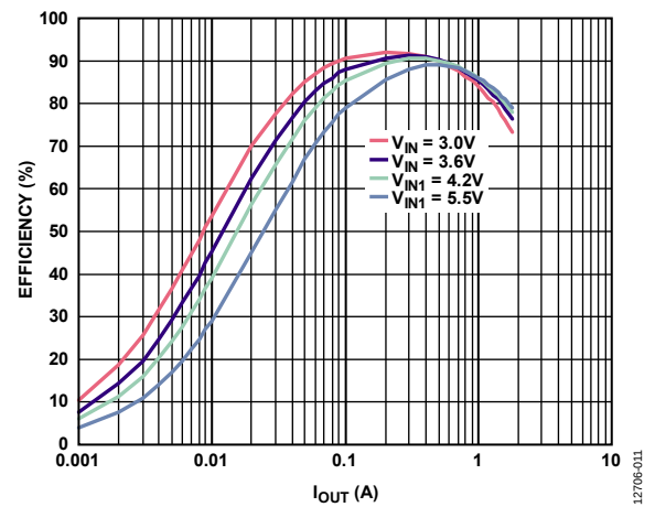
Figure 11. Buck2 FPWM Efficiency, Across V_{IN} , V_{OUT2} = 1.8\text{V}
