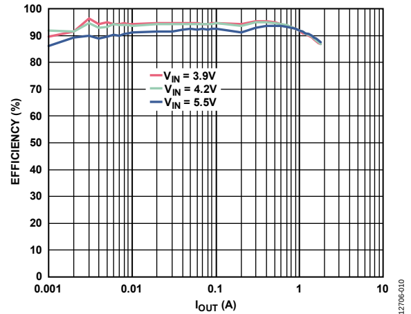
Figure 10. Buck1 PSM Efficiency, Across V_{IN} , V_{OUT1} = 3.3\text{V}
