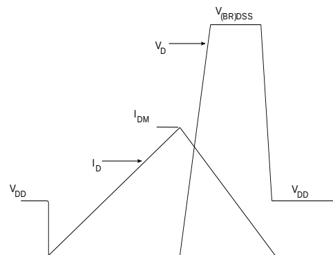
Figure 17: Unclamped inductive waveform
