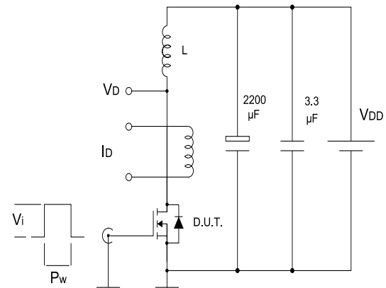
Figure 16: Unclamped inductive load test circuit
