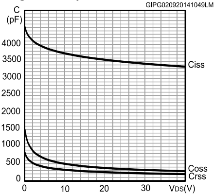
Figure 8: Capacitance variation
