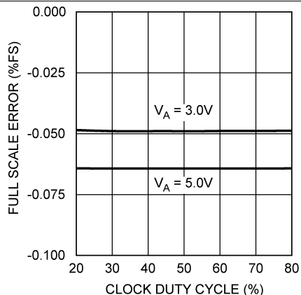
Figure 27. Full-Scale Error vs. Clock Duty Cycle
