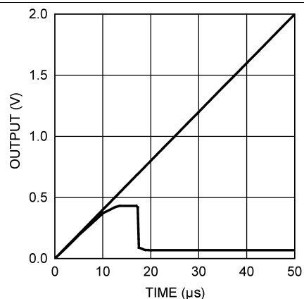
Figure 32. Power-On Reset
