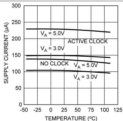
Figure 30. Supply Current vs. Temperature
