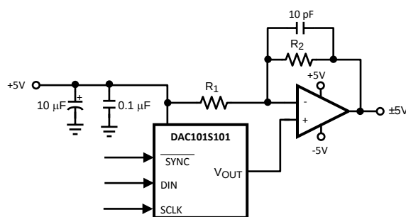
Figure 41. Bipolar Operation
