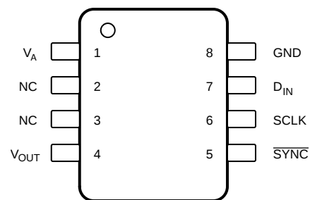
DAC101S101 DGK Package 8-Pin (VSSOP) Top View
