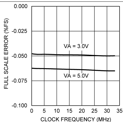
Figure 26. Full-Scale Error vs. f_{SCLK}
