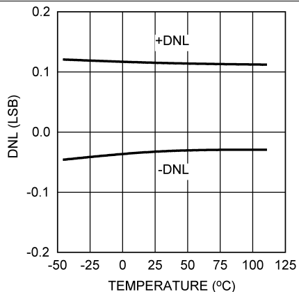
Figure 15. 3-V DNL vs. Temperature
