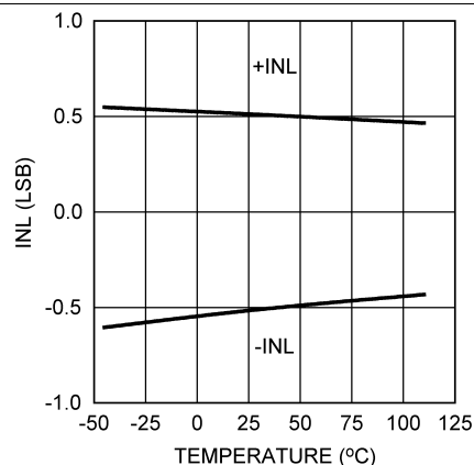
Figure 22. 5-V INL vs. Temperature
