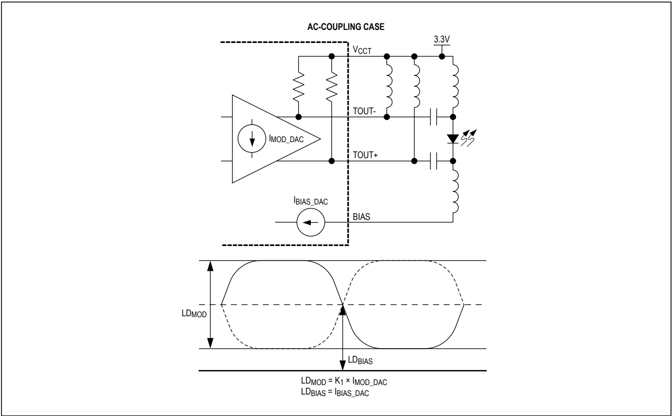
Figure 1. AC-Coupling Case
