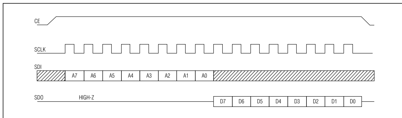
Figure 8. SPI Single-Byte Read
