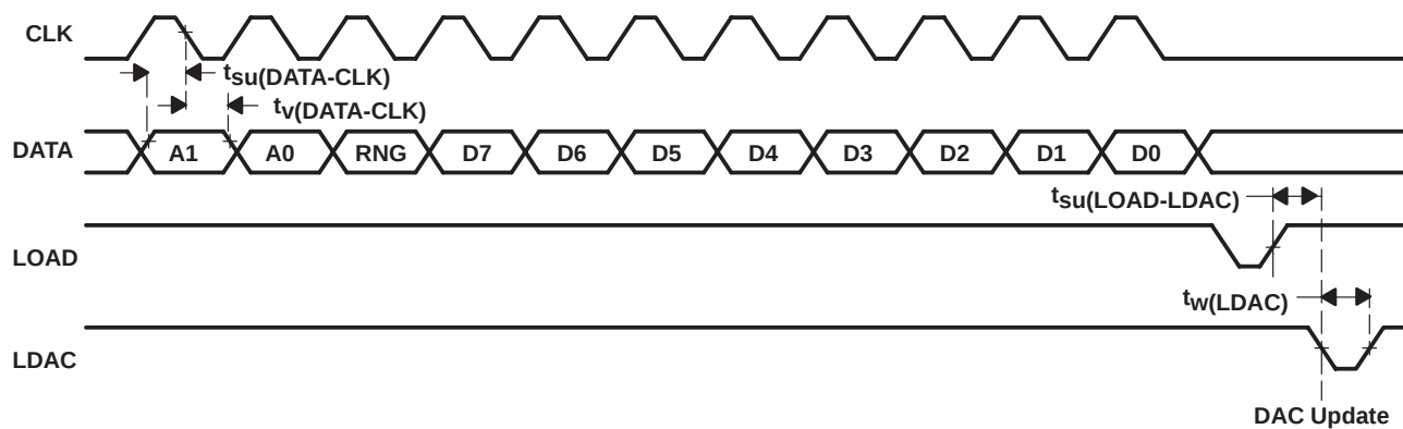
Figure 2. LDAC-Controlled Update
