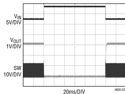
V_{IN} Overvoltage
