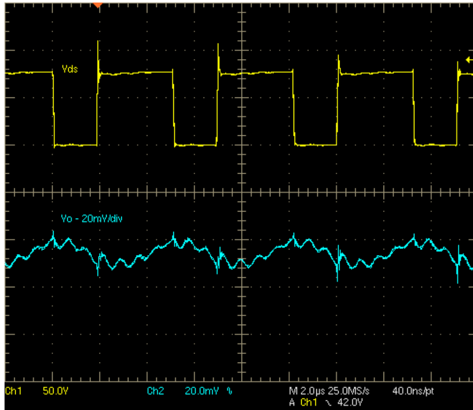
Figure 5. Output Voltage Ripple (48Vin 8A)
