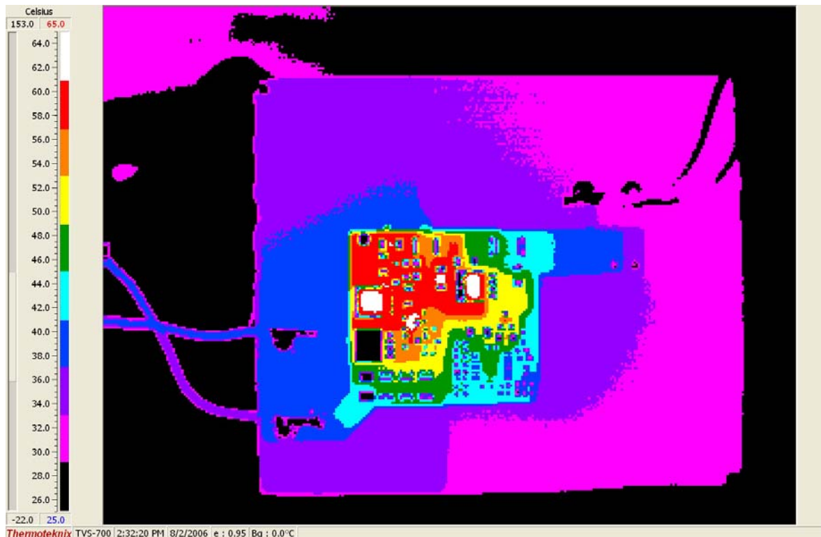
Figure 8. Temp Data (48Vin, 8A, 100LFM airflow – back)
