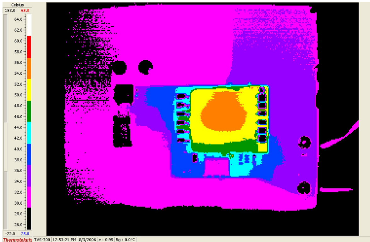
Figure 7. Temp Data (48Vin, 8A, 100LFM airflow – front)
