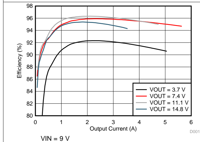
Figure 5. System Efficiency
