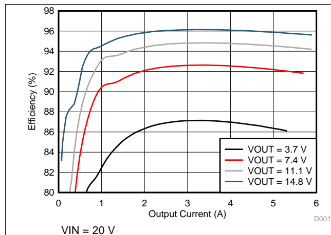
Figure 7. System Efficiency
