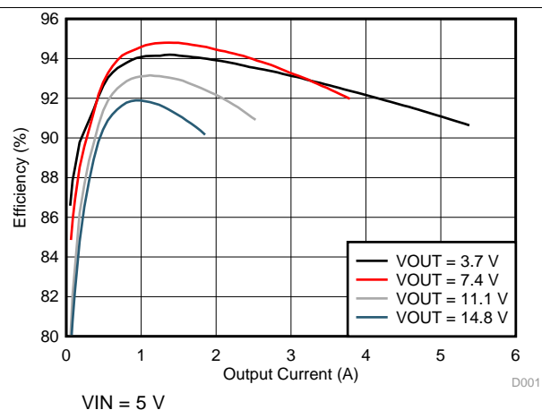
Figure 4. System Efficiency
