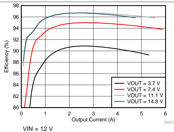
Figure 6. System Efficiency
