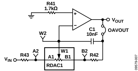
Figure 7. Pseudologarithmic Inverting Amplifier
