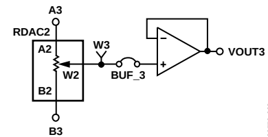
Figure 8. RDAC2
