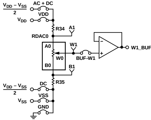
Figure 2. DAC
