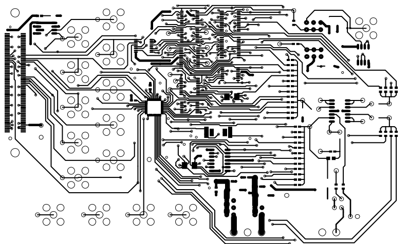
Figure 18. Component Placement Drawing
