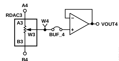
Figure 9. RDAC3
