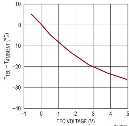
TEC Temp vs TEC Voltage (VIN = 12V)*
