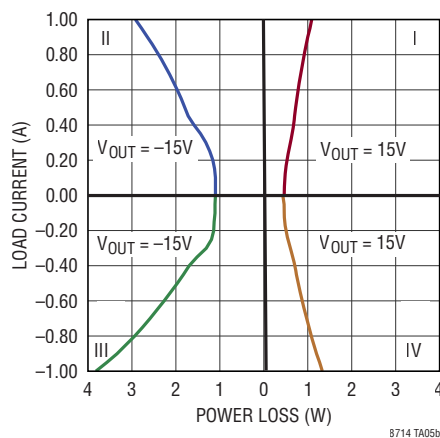
Power Loss in Each Quadrant ( V_{IN} = 24V )
