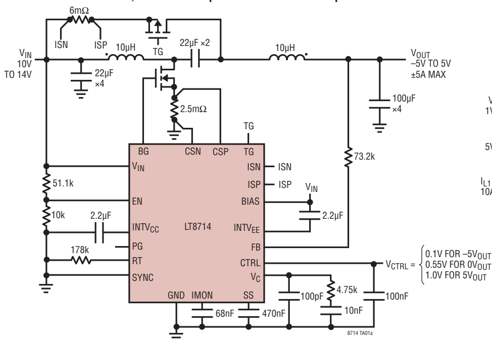
200kHz, -5V to 5V Output from a 10V to 14V Input
