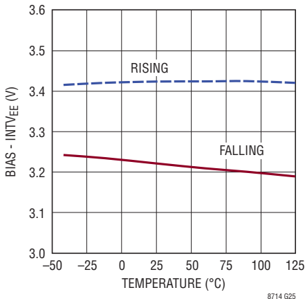
INTV EE UVLO vs Temperature
