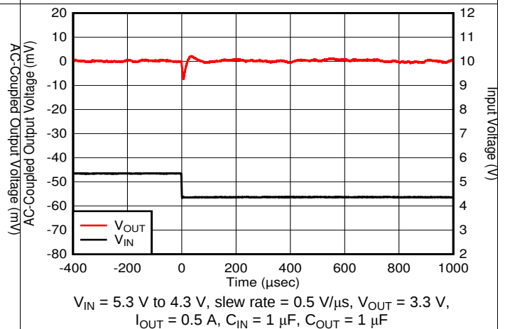
Figure 30. Line Transient
