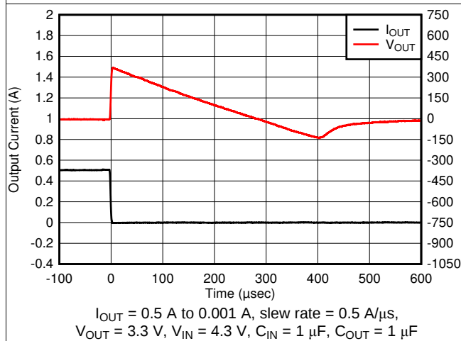
Figure 29. Load Transient
