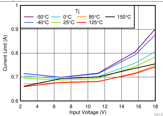
Figure 8. Current Limit vs V_{IN}
