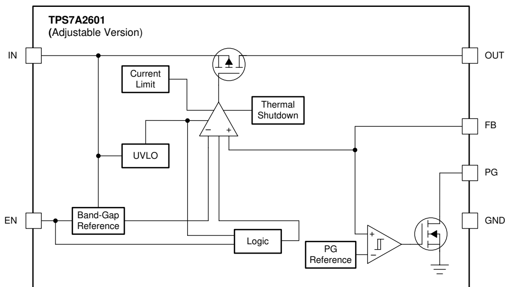
Figure 34. Adjustable Version
