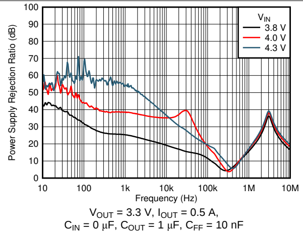
Figure 20. PSRR vs Frequency and V_{IN}
