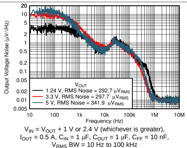
Figure 24. Output Noise ( V_n ) vs Frequency and V_{OUT}
