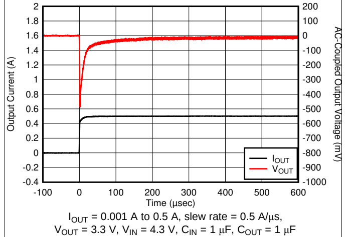
Figure 28. Load Transient
