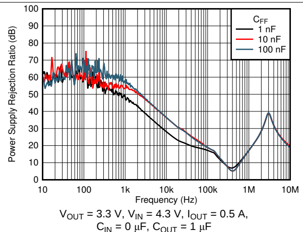
Figure 22. PSRR vs Frequency and C_{FF}
