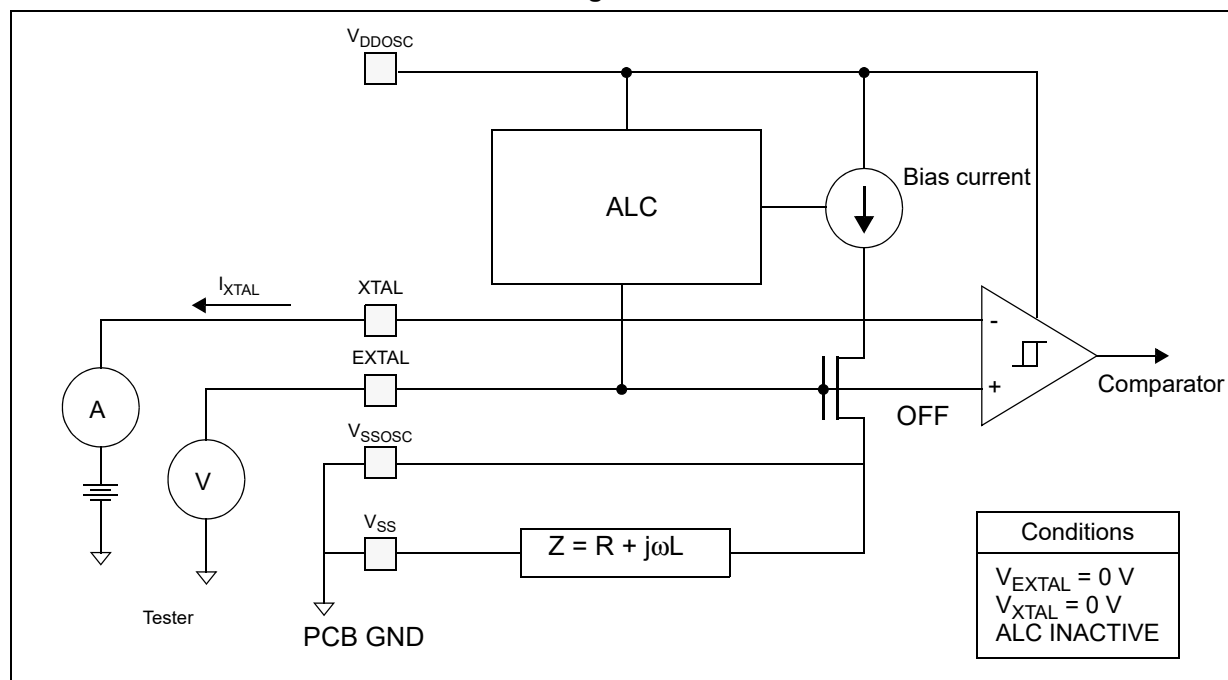
Figure 12. Test circuit
