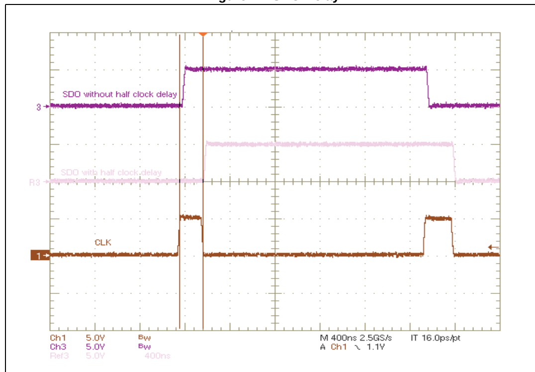
Figure 11. SDO Delay
