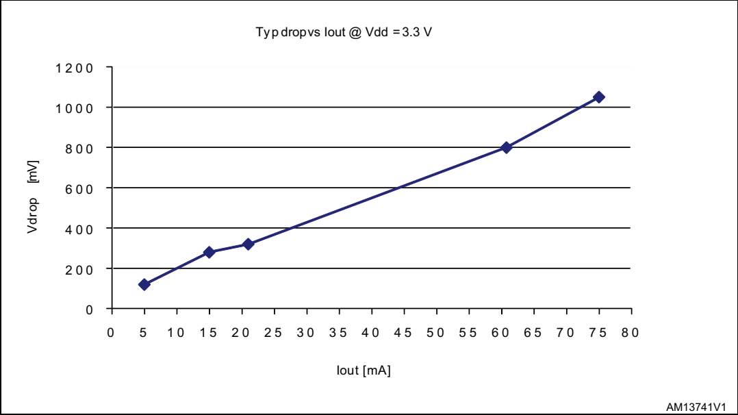
Figure 18. Typical dropout voltage vs. output current (only one channel ON)
