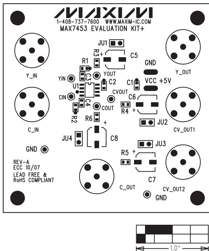
Figure 2. MAX7453 EV Kit Component Placement Guide—Top Silkscreen
