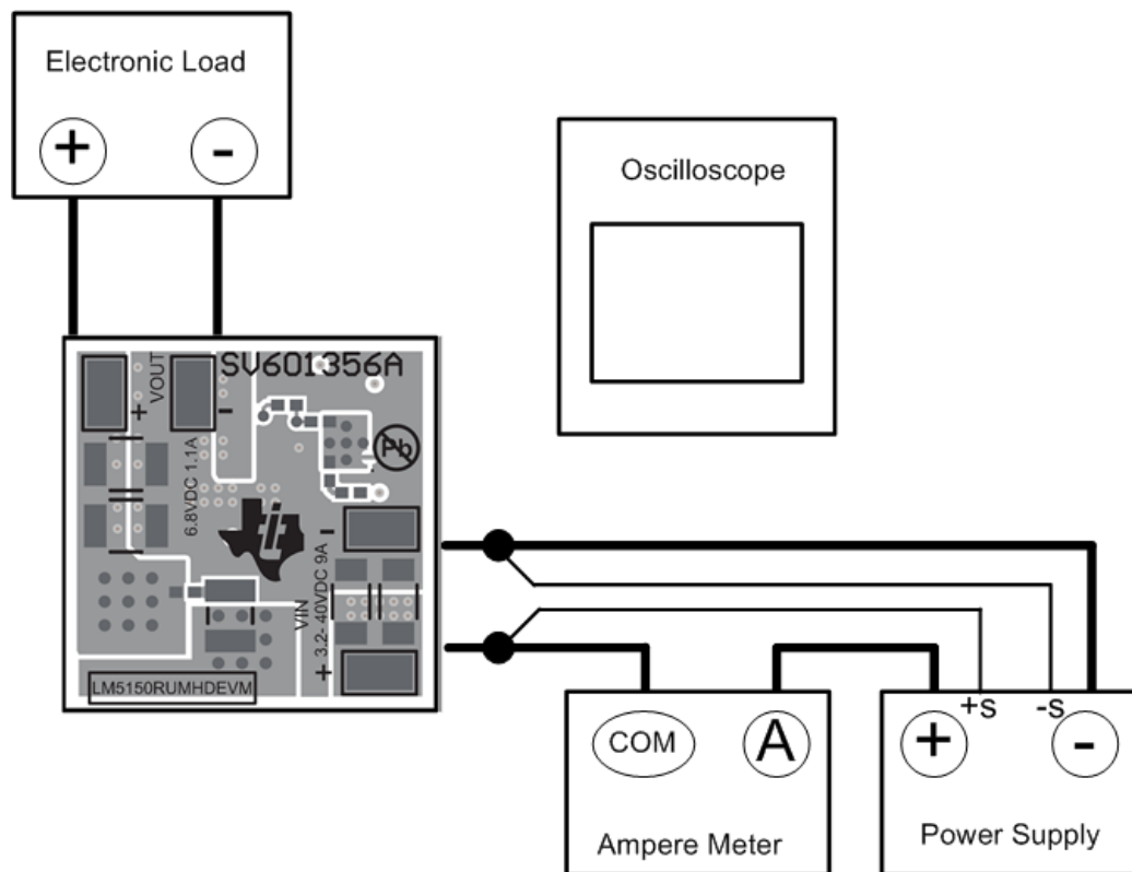
Figure 1. Standard Connection Diagram
