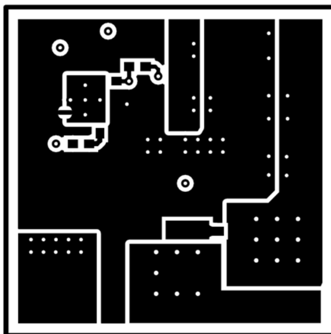
Figure 12. Bottom Copper (X-Ray View)
