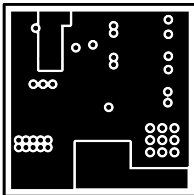
Figure 10. Mid1 Copper (X-Ray View)
