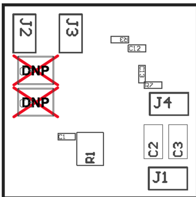
Figure 14. Bottom Assembly (Bottom View)
