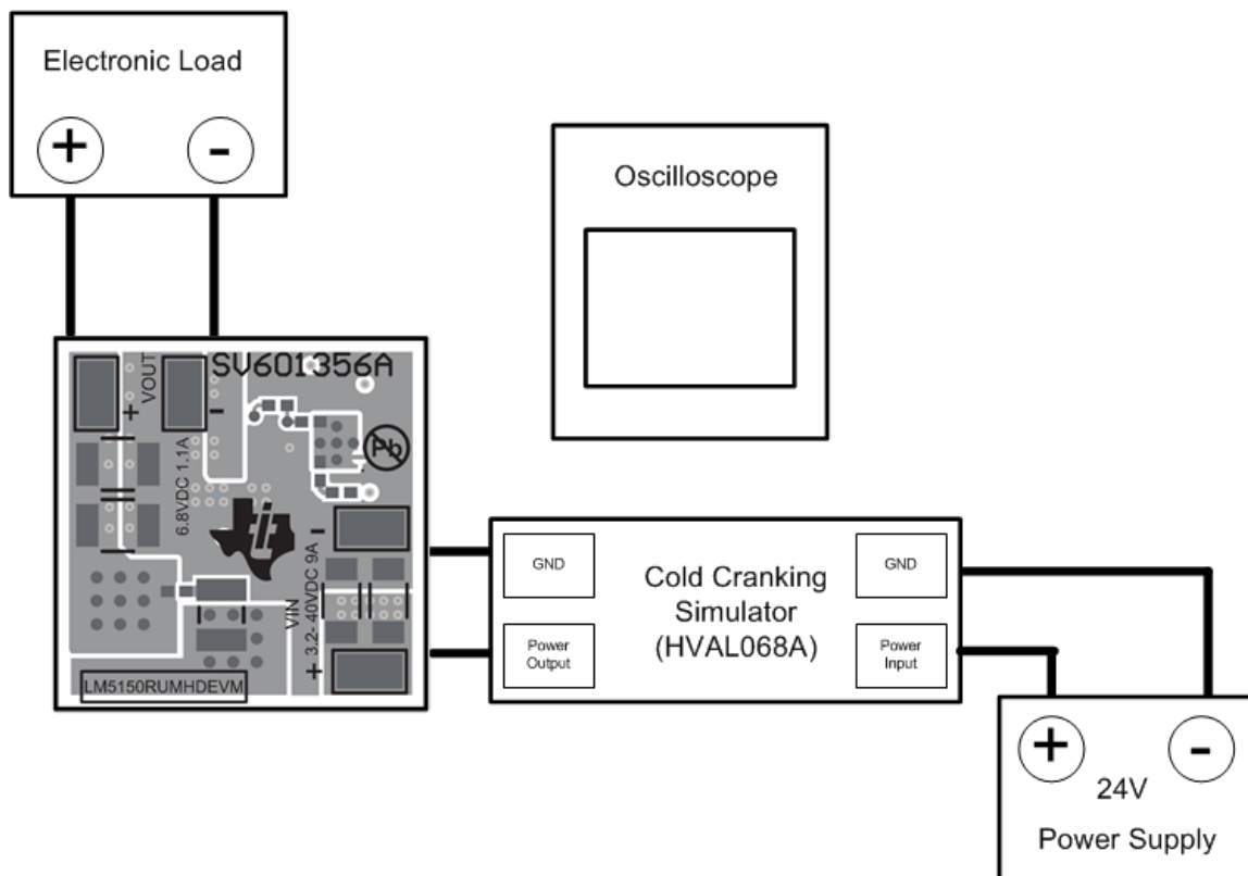
Figure 2. Cranking Simulator Connection Diagram
