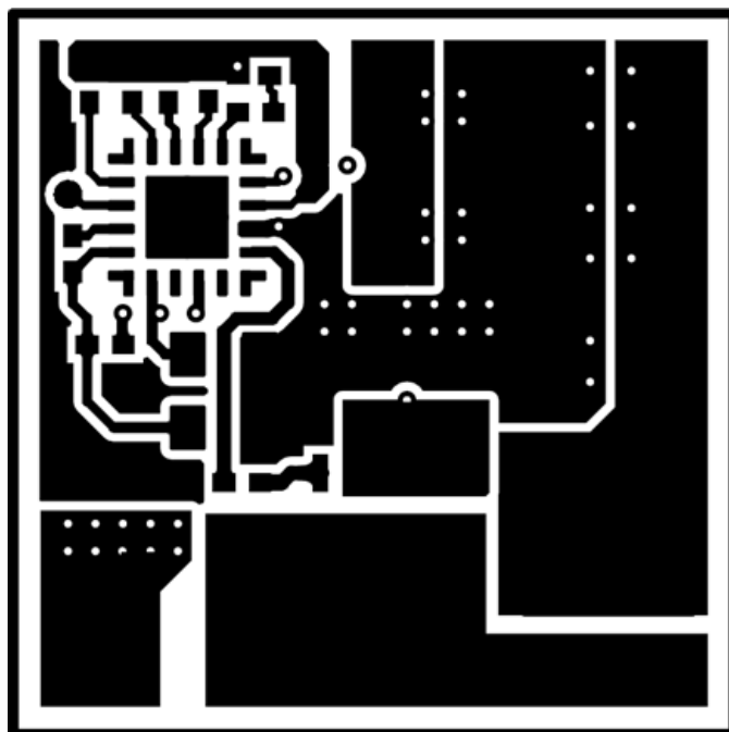
Figure 9. Top Copper (Top View)
