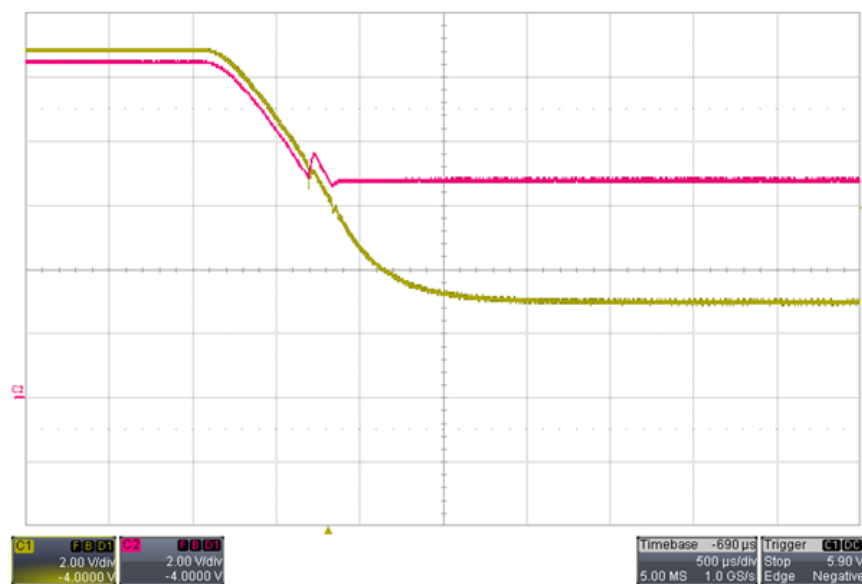
Figure 4. Cold-Cranking Using Cranking Simulator(C1:V_SUPPLY, C2:V_LOAD)
