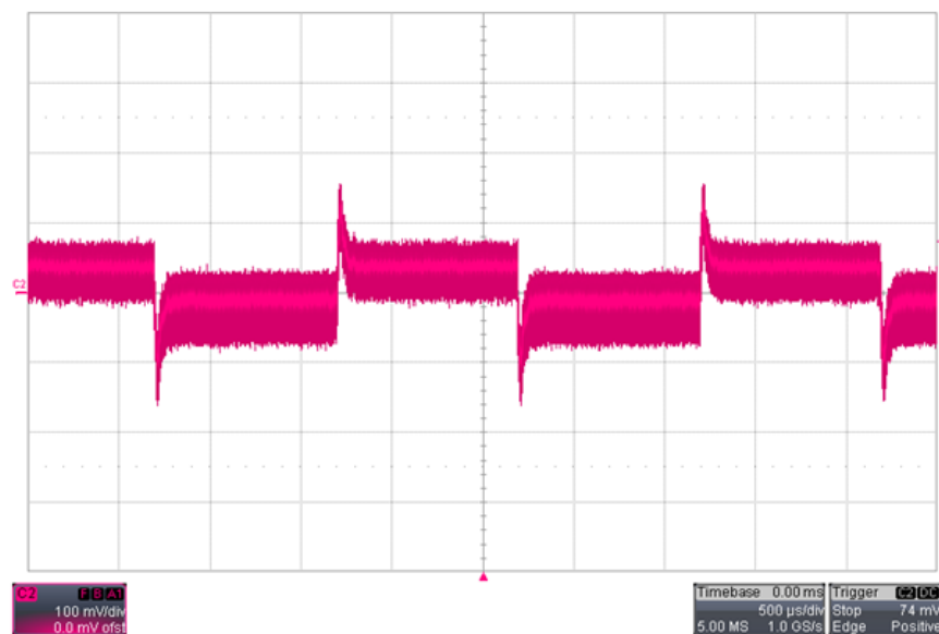
Figure 5. Load Transient(C2: V_{LOAD} AC-coupled)
