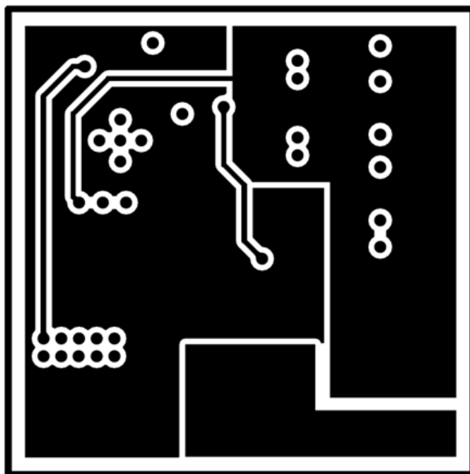
Figure 11. Mid2 Copper (X-Ray View)
