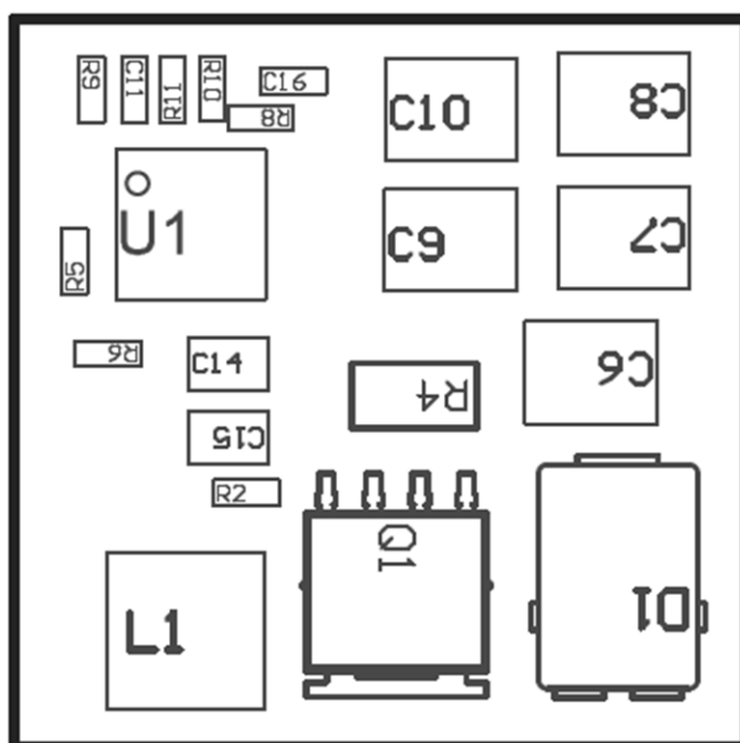
Figure 13. Top Assembly (Top View)
